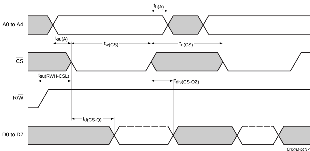
Fig 12. General read timing in 68 mode
