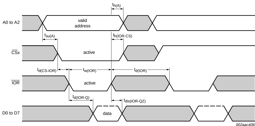
Fig 11. General read timing in 16 mode
