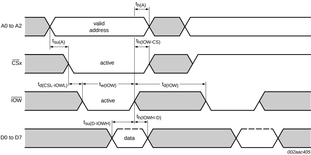
Fig 9. General write timing in 16 mode
